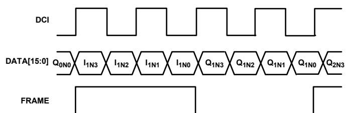
Figure 45. Timing Diagram for Nibble Mode
