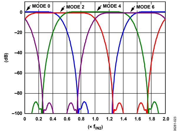
Figure 54. HB2, Even Filter Modes
