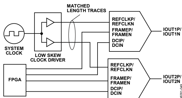
Figure 82. Typical Circuit Diagram for Synchronizing Devices
