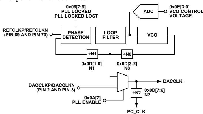
Figure 65. PLL Clock Multiplication Circuit
